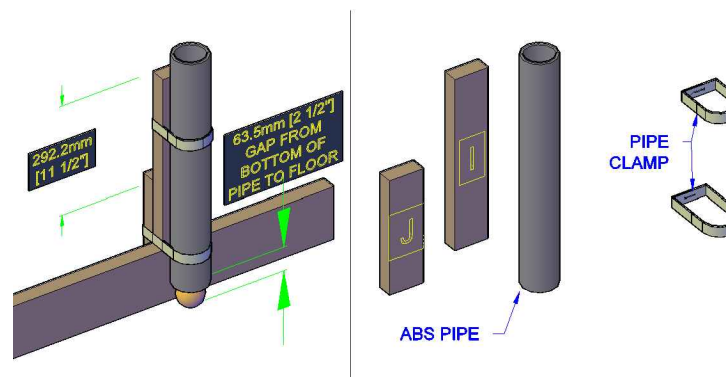
③ BALL DISPENSER DETAILS (EXPLODED) SCALE = N.T.S.
