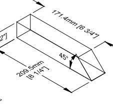
⑧ T DIMENSIONS SCALE = N/A
