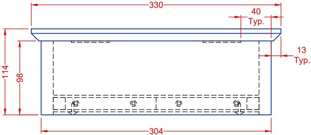
FRONT
