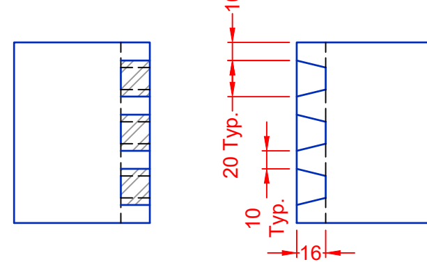
Secondary Through Dovetail - Do NOT glue
