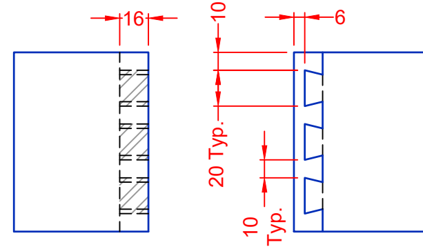
Secondary Through Dovetail - Do NOT glue
