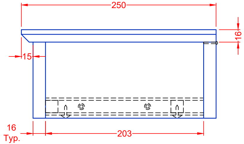
SIDE
