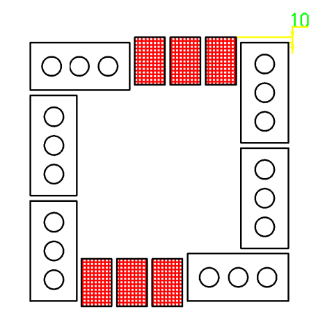
VIEW B BRICK 3RD COURSE LAYOUT
