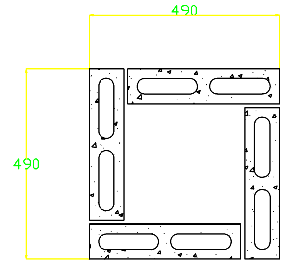
VIEW A BLOCK LAYOUT
